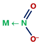
Nitro / Nitrito-N
