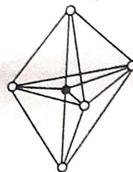
Trigonal bipyramid
