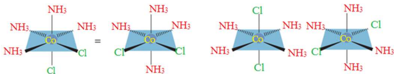
Cis - Isomer
