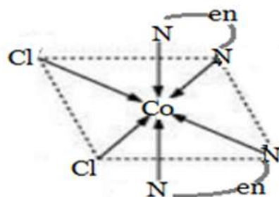
leavo - form
