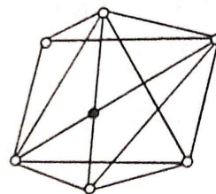
Octahedral
